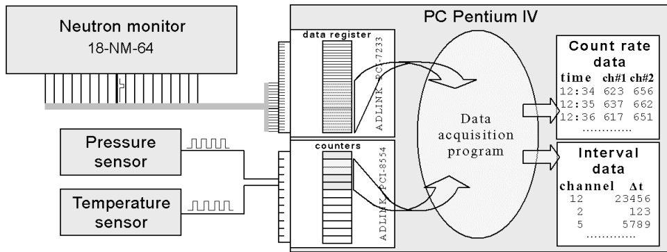
Fig.1. The new data acquisition system at the neutron monitor station Barentsburg
